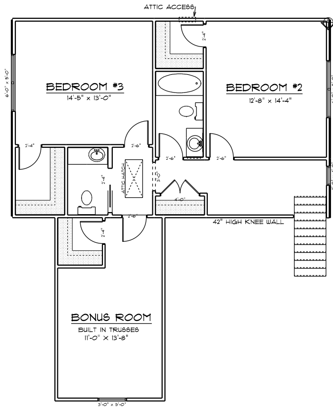
2ND FLOOR
